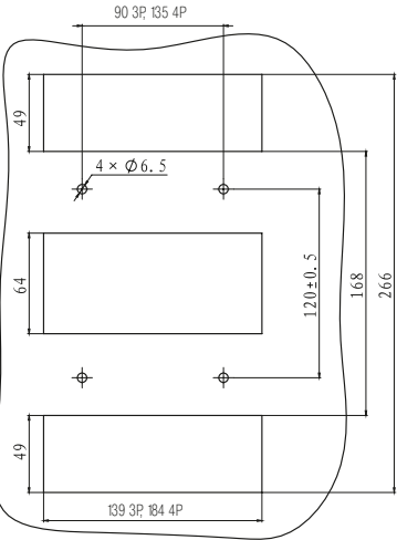
BA57 Aksol 400AF/630AF
